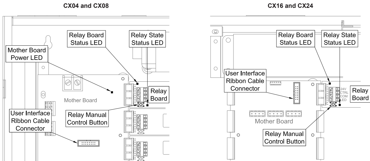
Figure 4 - Panel Start-Up Controls
