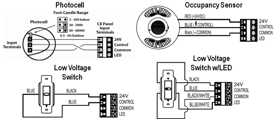
Figure 3 - Low Voltage Input Wiring Diagrams
