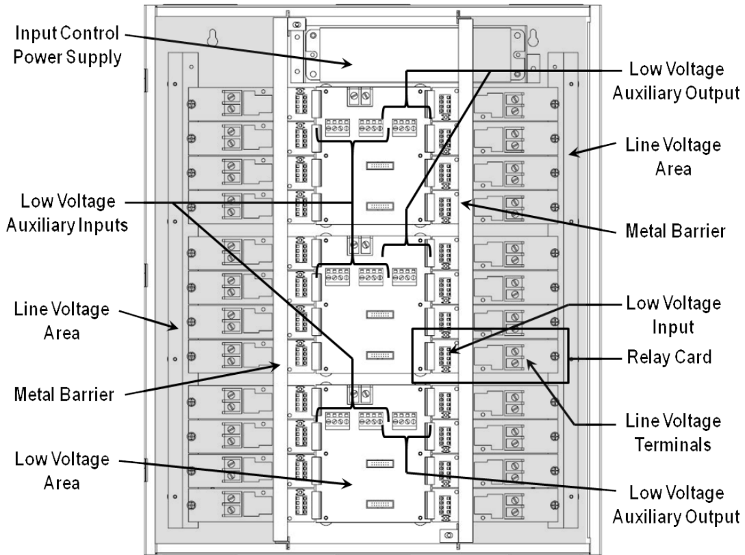
Figure 1(b) – CX16 or 24 Panel Interior
