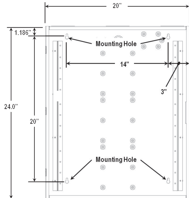
Figure 2(b) - Enclosure Mounting Holes 16/24 Panels
