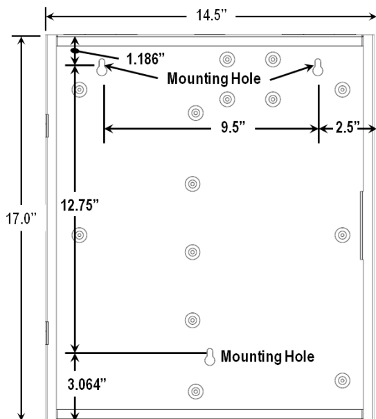
Figure 2(a) - Enclosure Mounting Holes - 4/8 Panels
