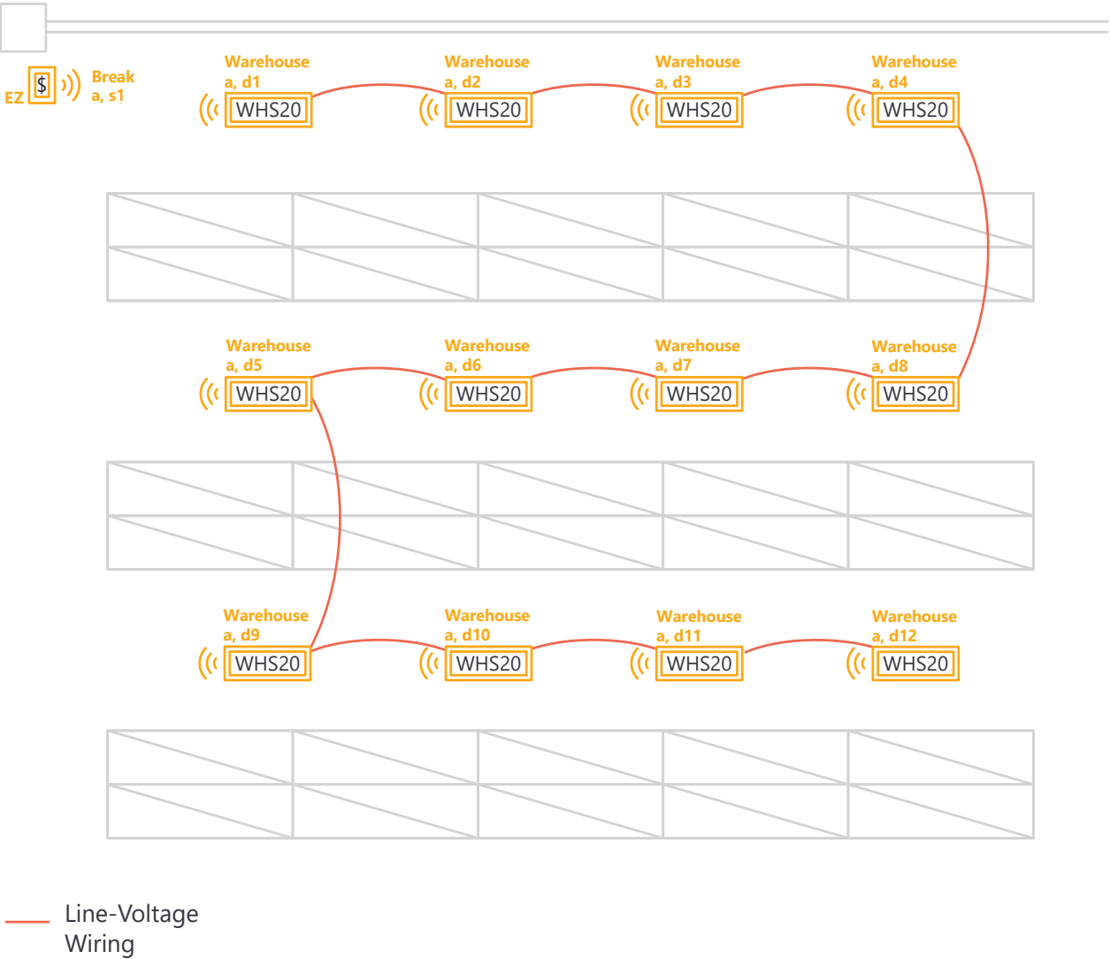
Warehouse Daintree EZ Connect 12-WHS20-High bay fixture control with daylight and occupancy
