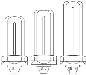
F26TBX F32TBX F42TBX GX24q-3 GX24q-3 GX24q-4
