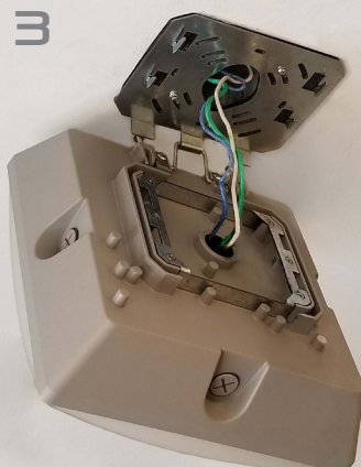
3 Complete wiring connections.
