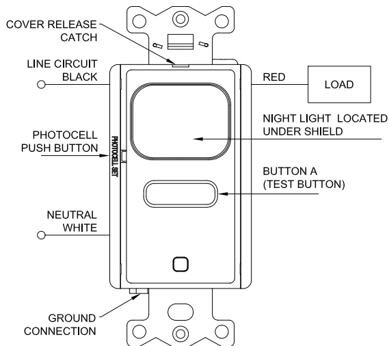
FIGURE 1 - WIRING DIAGRAM
