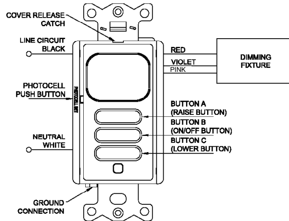
FIGURE 1 - WIRING DIAGRAM
