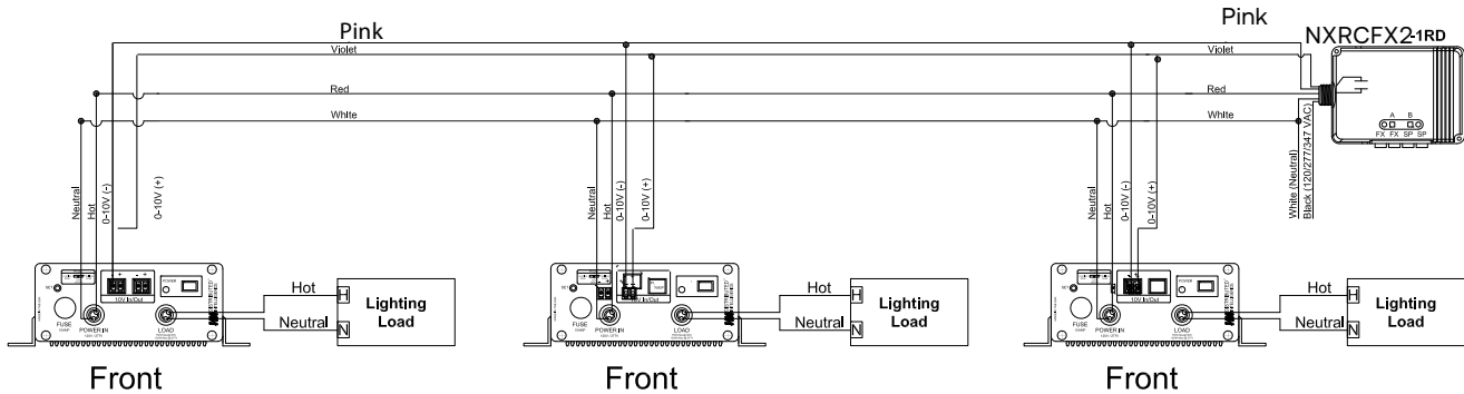
FIGURE 2: Wiring Diagram to multiple NXFRD
