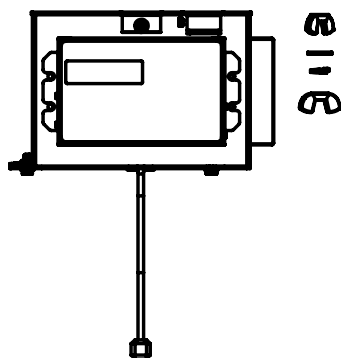
J-box/Cable Kit Assembly with mounting hardware SCALE 1 : 5
