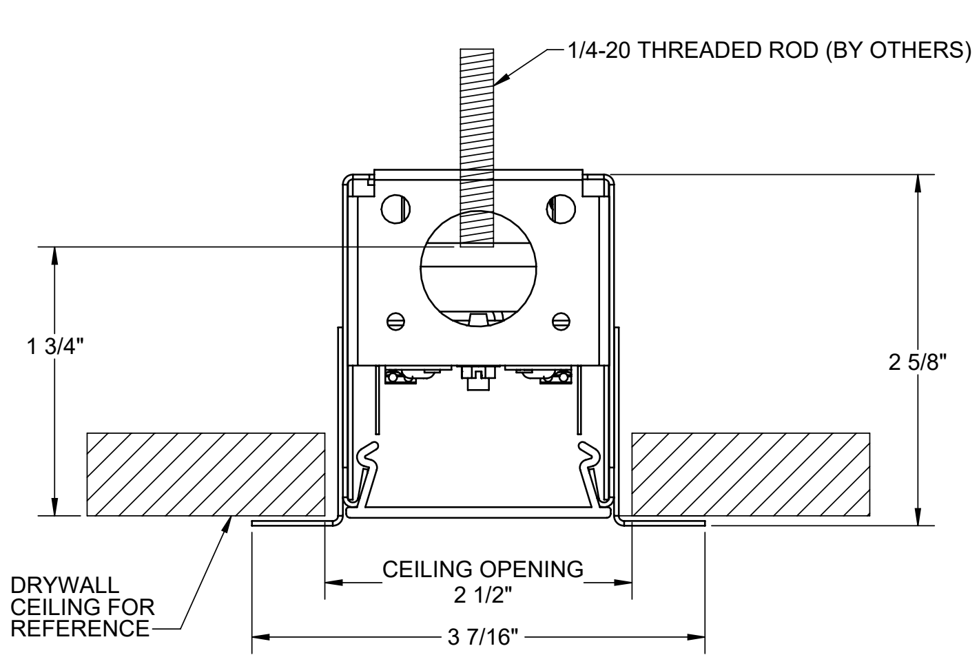
2L-DW CROSS SECTION
