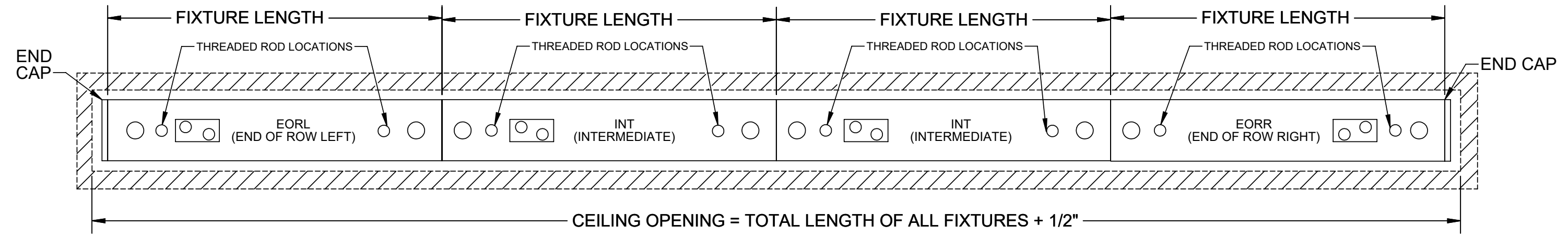
TOP VIEW - ROW MOUNTED RECESSED FIXTURE
