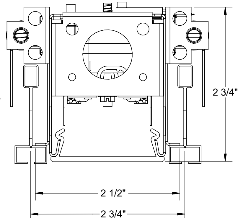
SS-D (SCREWSLOT) CROSS SECTION
