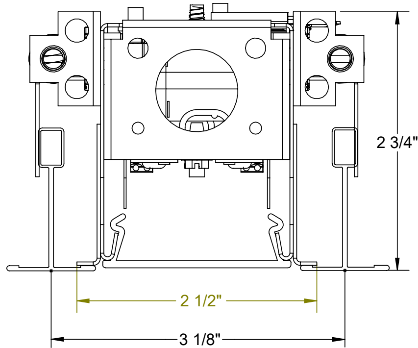
LG-D (15/16") CROSS SECTION
