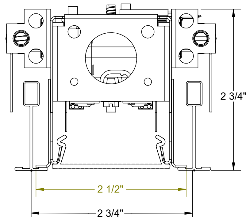
NG-D (9/16") CROSS SECTION
