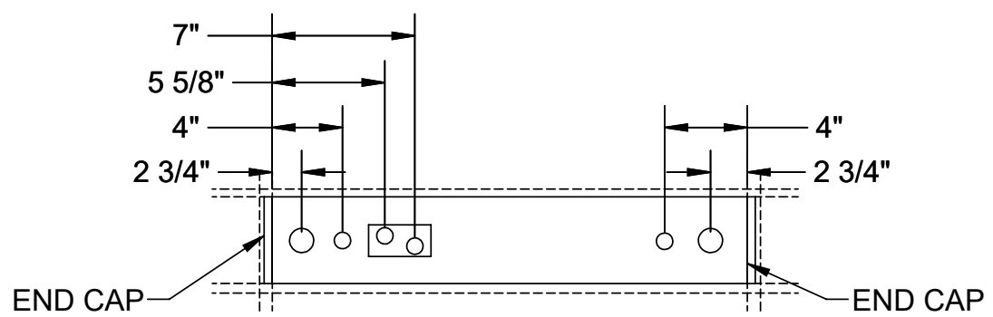
TOP VIEW - INDIVIDUALLY MOUNTED RECESSED FIXTURE
