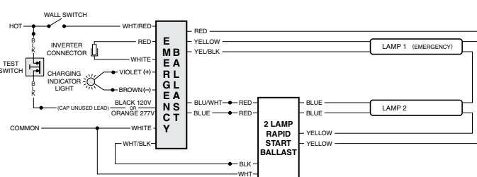
FIG L TWO (2) LAMP PROGRAM RAPID START OSRAM BALLAST
