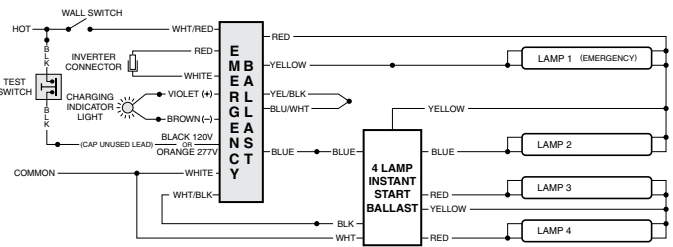
FIG J FOUR (4) LAMP INSTANT START BALLAST
