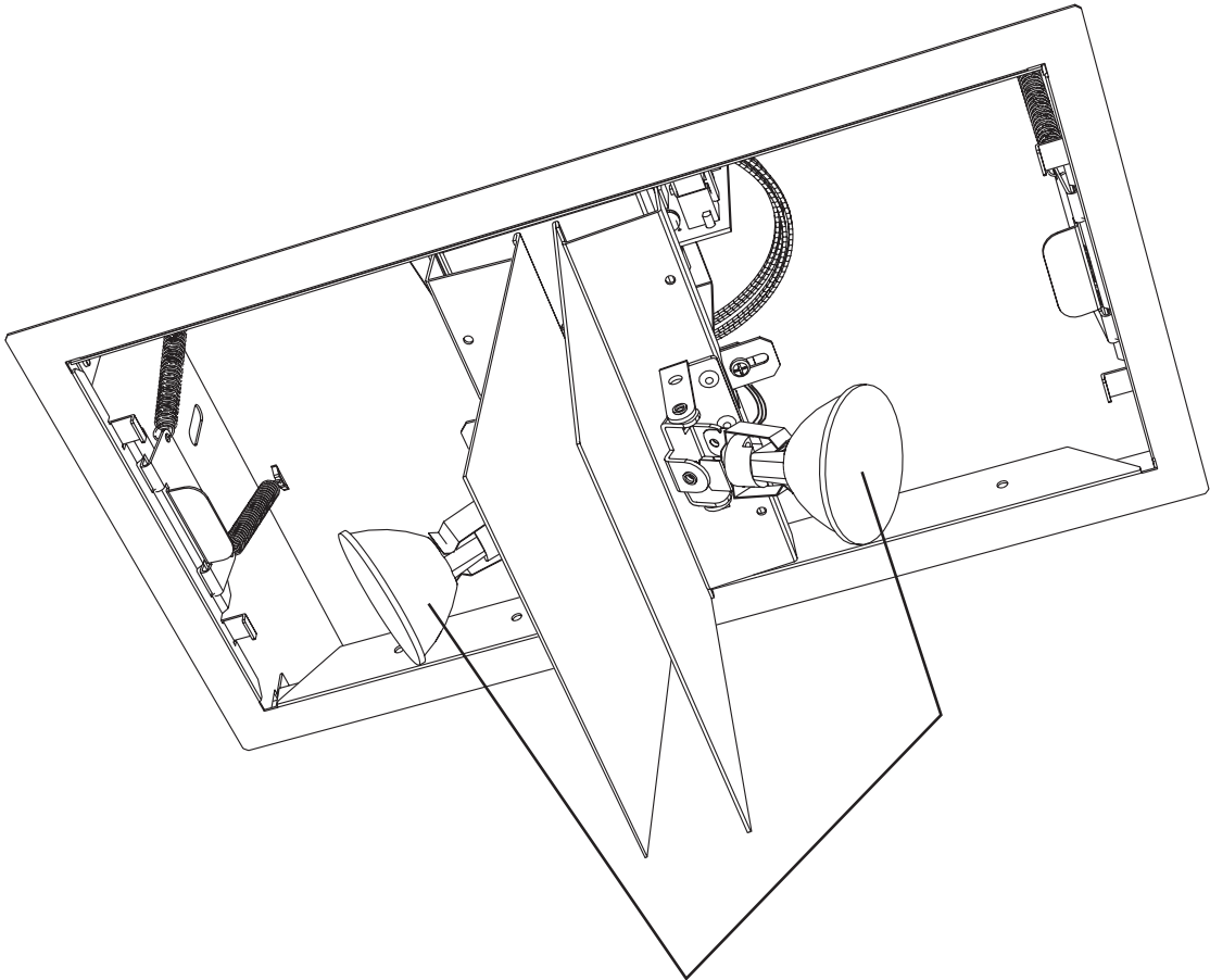
Adjustable Lampholder
