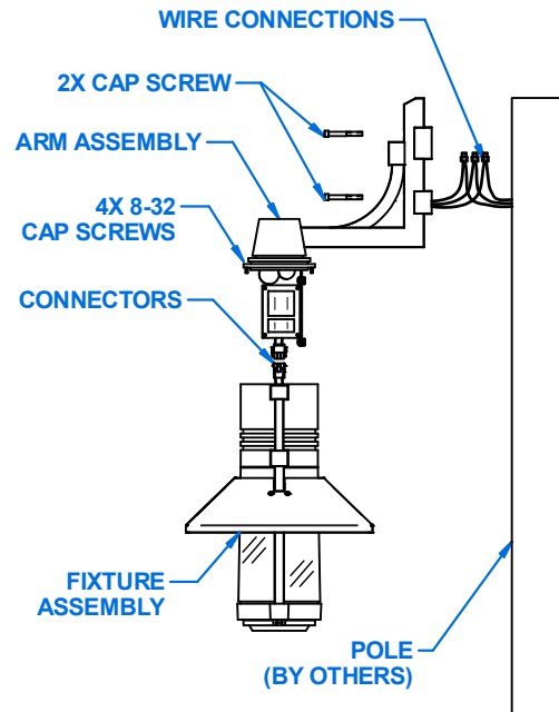
PSA-BD/BU
