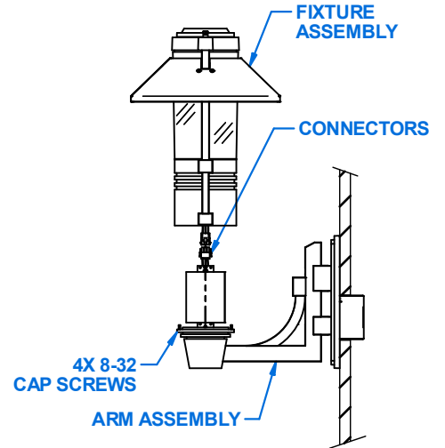
FIXTURE ASSEMBLY
