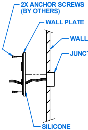
WALL PLATE
