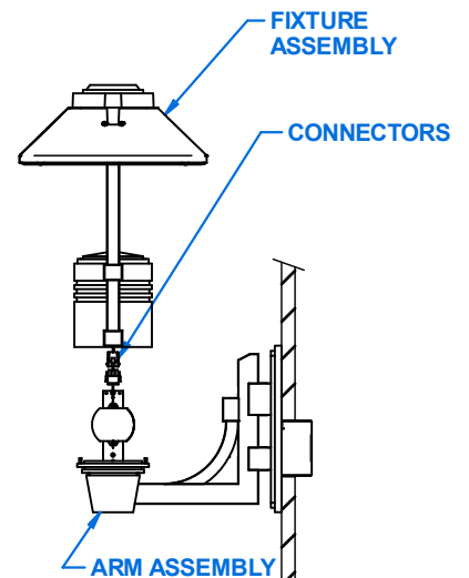
FIXTURE ASSEMBLY
