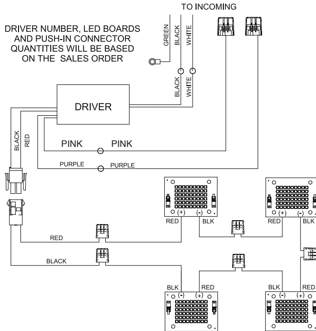
WIRING DIAGRAM
