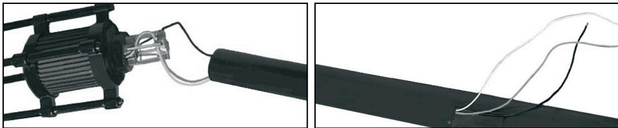
1. Feed fixture wires down pole and out hand hole.
