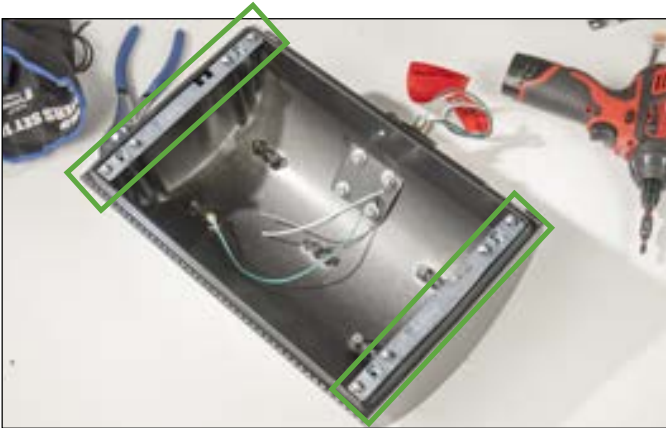
13. Place new mounting brackets from packet of parts. Secure using 8 philips head screws.
