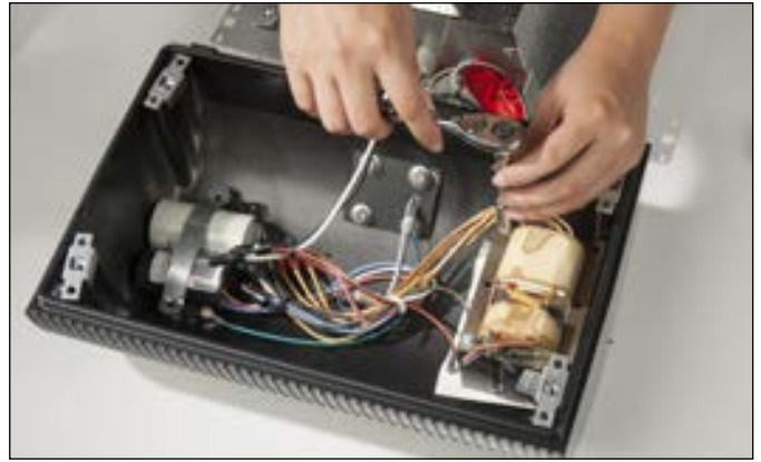
10. Using pliers, remove 2 nuts holding ballast into place.
