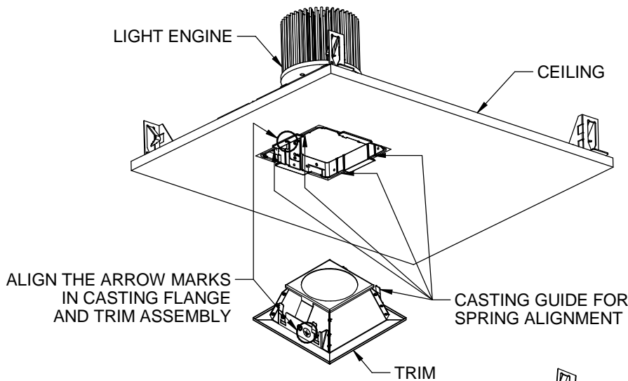
FIG 1.1 STANDARD/SHALLOW DOWNLIGHT
