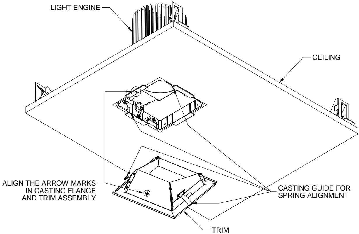
FIG 3.1 ADJUSTABLE DOWNLIGHT
