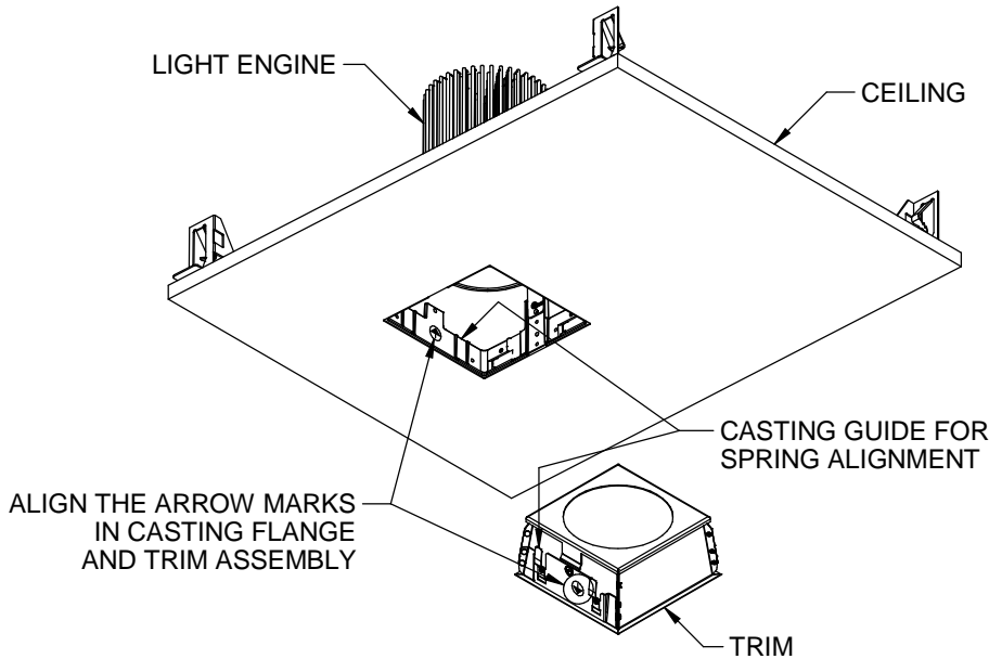
FIG 2.1 STANDARD/SHALLOW DOWNLIGHT
