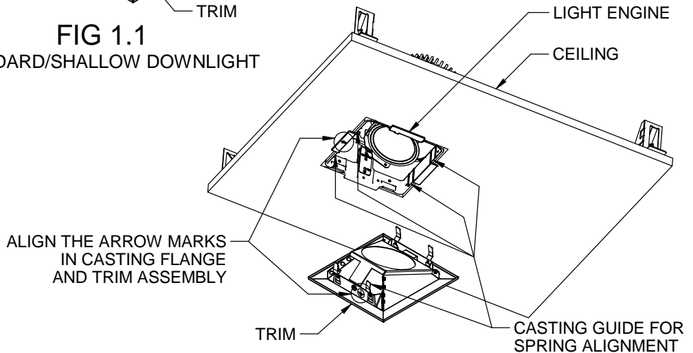
FIG 1.2 LWW DOWNLIGHT
