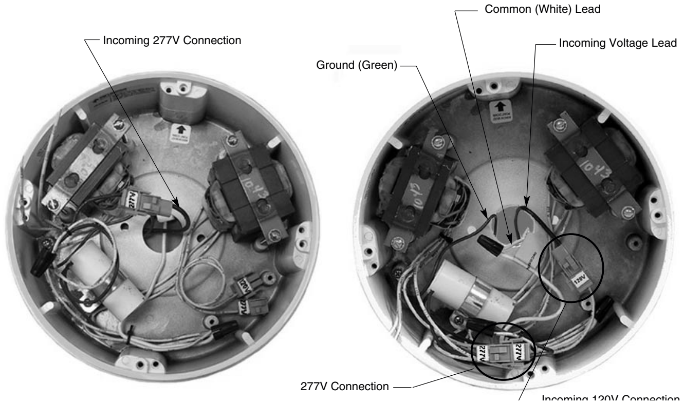
Pre-Wired 277 Voltage Figure 1
