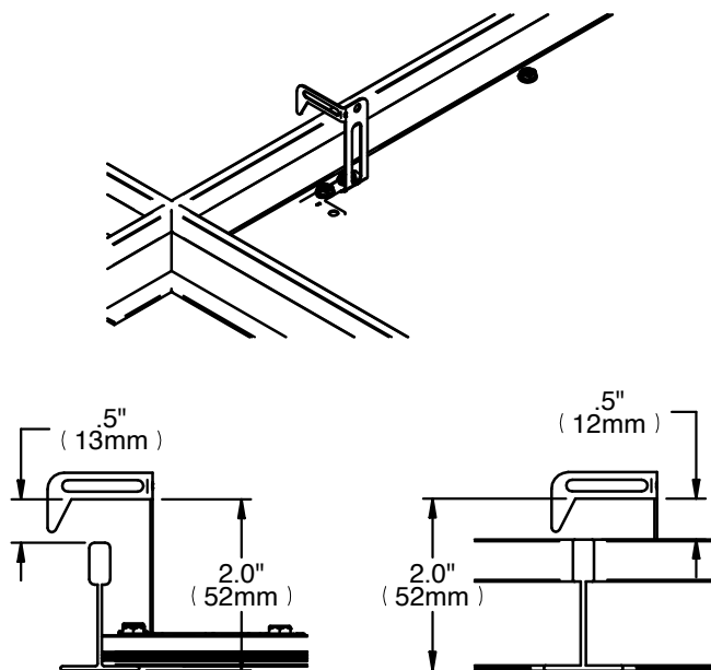
Figure 1B T-Grid Install
