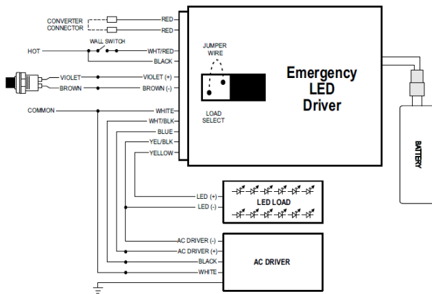
Figure 6 2-Wire Integrated Test Switch
