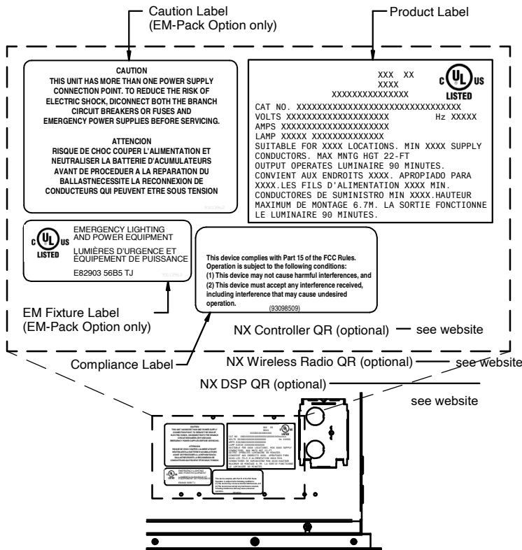
Figure 1A Labeling detail
