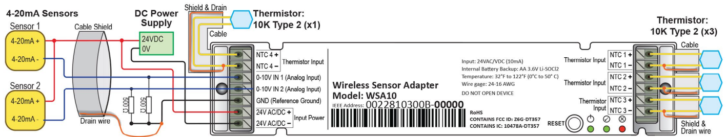
Figure 6: WSA10 terminal connections for 4-20mA sensors and NTC thermistors, using a DC Power Supply adaptor for DC Power Supply
