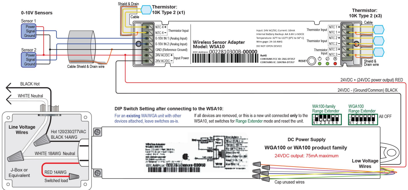
Figure 4: WSA10 terminal connections for 0-10V sensor and NTC thermistors, using a WGA100 or WA100-family adaptor for DC Power Supply
