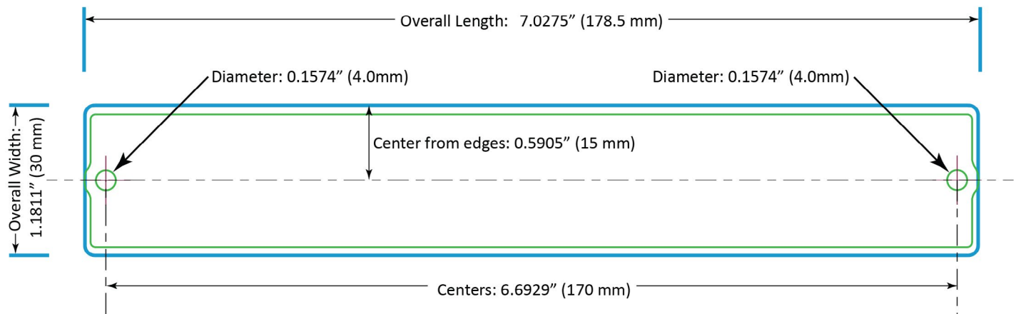
Figure 8: Mounting Template (observe measurements, illustration may not be actual size).for DC Power Supply
