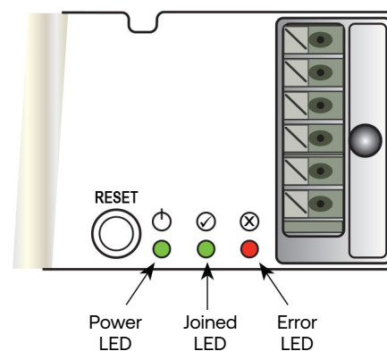
Figure 1: LED indicators
