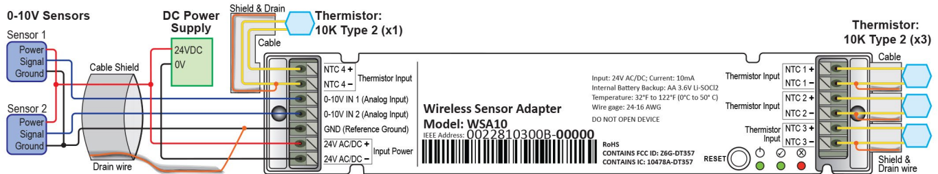
Figure 2: WSA10 terminal connections 0-10V sensors and NTC thermistors, using a DC Power Supply
