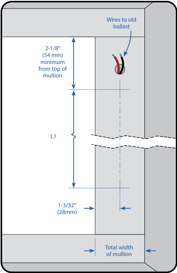
1 Mark two hole locations on mullion.
