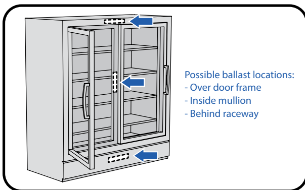
④ Locate ballast and remove access cover.
