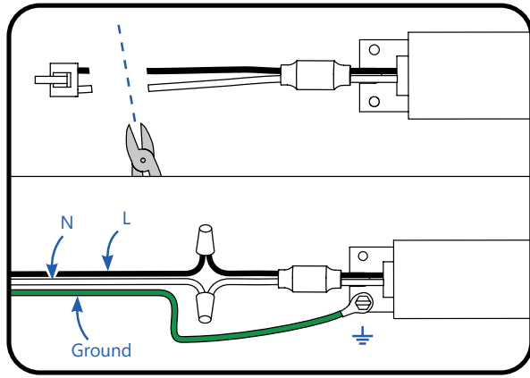
(B) Connect AC input using wire nuts.
