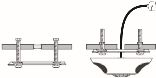
Mounting Method 1: Screw and mount twist-lock cover plate.
