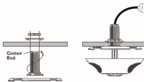
Mounting Method 2: Twist and lock threading mounting post into cover plate. Drill into ceiling tile.
