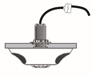
Run NXCBL-P2 through ceiling tile. Attach sensor body to cover plate by aligning arrows and twist locking into place. Connect cable to the mini SmartPort on sensor
