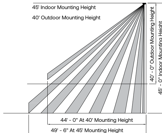
BTSMP-HMO Sensor Lens Coverage and Detection Patterns When Mounted at 40ft and 45ft with Standard Lens
