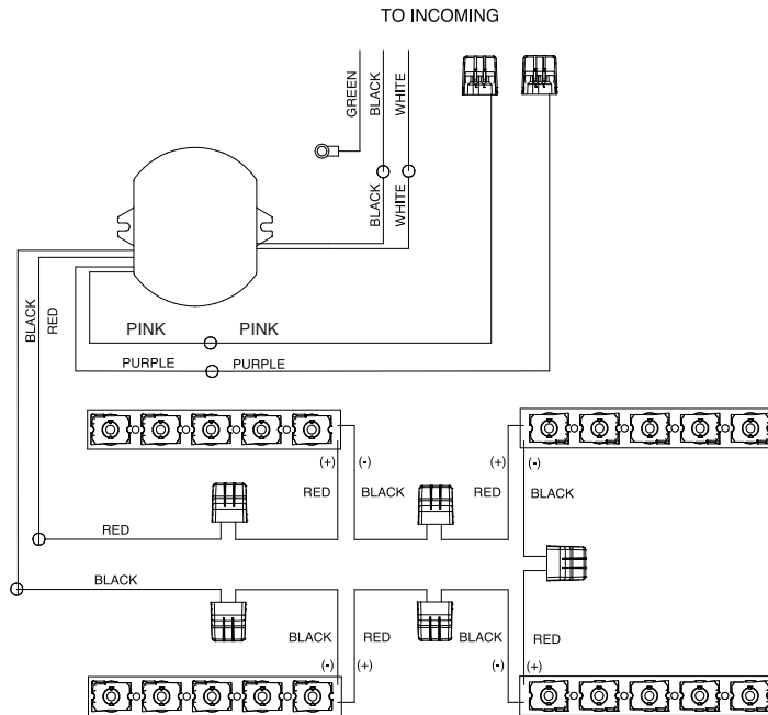
WIRING DIAGRAM
