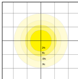
GSY-65-4K7 Scale: 1 = 20 ft. Mounting Height: 25 ft.
