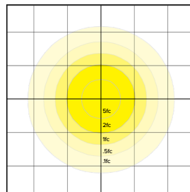
GSY-100-4K7 Scale: 1 = 20 ft. Mounting Height: 25 ft.
