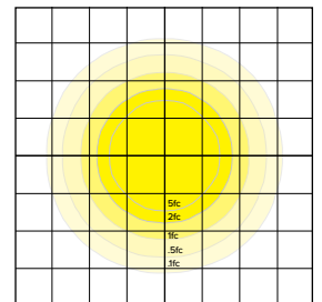
GSY-150-4K7 Scale: 1 = 20 ft. Mounting Height: 15 ft.
