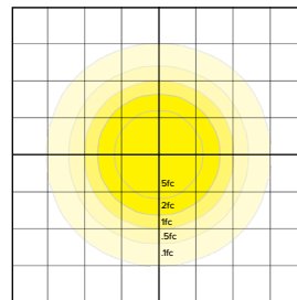
GSY-130-4K7 Scale: 1 = 20 ft. Mounting Height: 15 ft.
