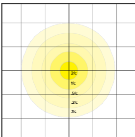
GSY-30-4K7 Scale: 1 = 20 ft. Mounting Height: 25 ft.
