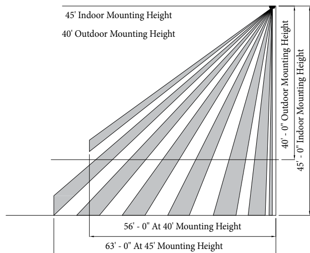
Sensor Lens Coverage and Detection Patterns When Mounted at 40ft and 45ft with Standard Lenses
