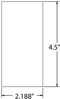
END CAP VIEW
