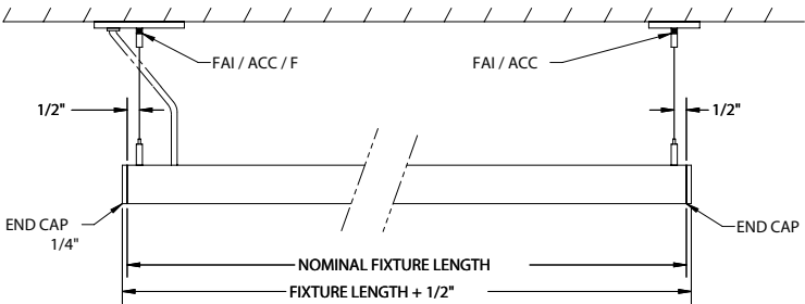
SIDE VIEW - INDIVIDUAL MOUNTED PENDANT MOUNTED FIXTURE INDIVIDUAL MOUNTING
