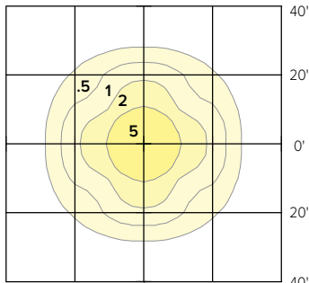
SGC-F-70-LSCS-UNVC @ 60W
