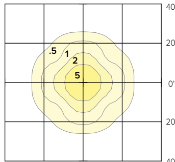
SGC-F-70-LSCS-UNVC @ 50W
