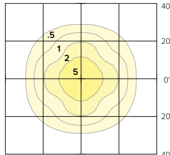
SGC-F-70-LSCS-UNVC @ 70W
