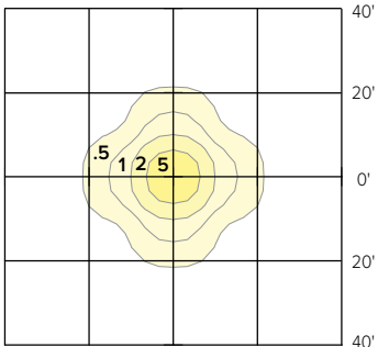
SGC-F-70-LSCS-UNVC @ 20W
