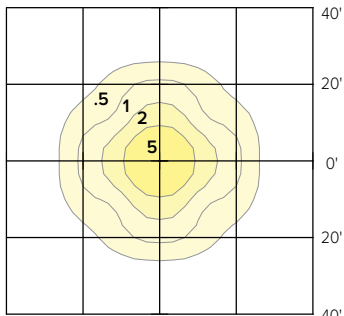
SGC-F-70-LSCS-UNVC @ 40W
