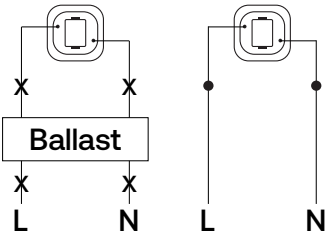
Wiring Diagram for G24d 2-pin Sockets
