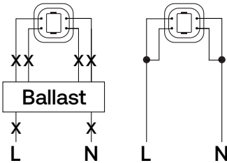
Wiring Diagram for G24q/GX24q 4-pin Sockets
