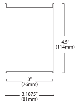
END CAP VIEW
