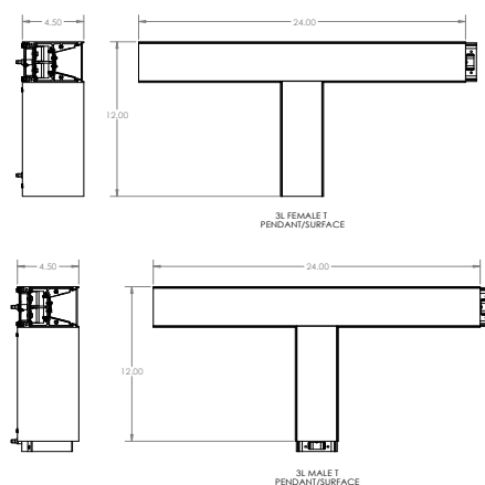
ROW MOUNTING
