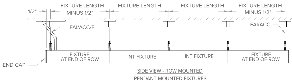
ROW MOUNTING
