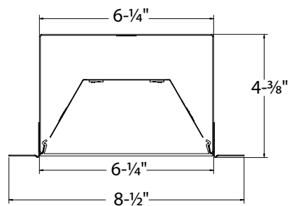
6L-PT
