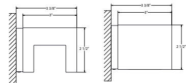
Cross Section Open End Cap
