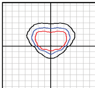
15' Mounting Height
