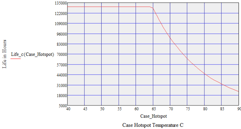
SLED 200W-XX-PCXXXX-RD Estimated Life Full Load @ 120Vac
