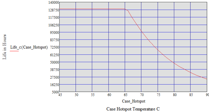
SLED40W Estimated Life Full Load @ 120Vac
