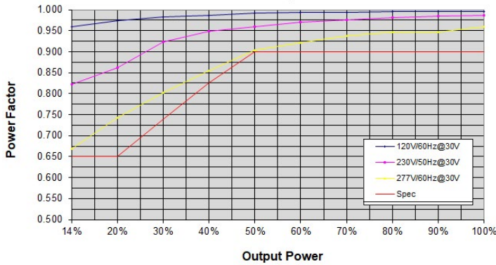
PF vs. Output Power
