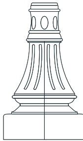
BC7-4/BC7-5 18" DIA x 30" high. Two piece clamshell with a one piece upper collar.
