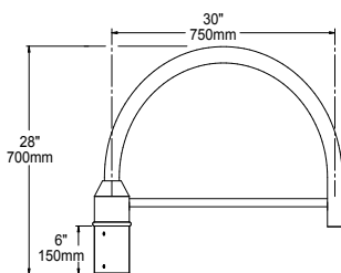
SLA18 (4" pole)
