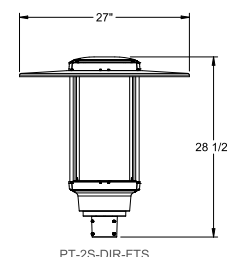
Slide Post Top Mount
