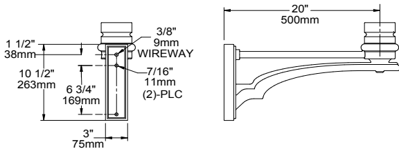
TRA55 (4" or 5" pole)
