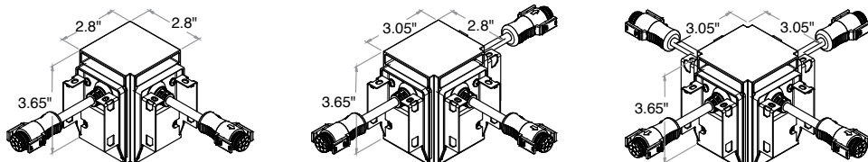
Connectors for the RND, Direct (Down)
