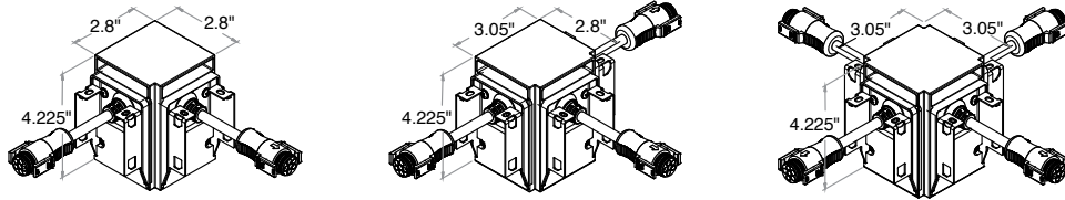
Connectors for the RND, Bidirectional (Up and Down) and RNI (Up)
