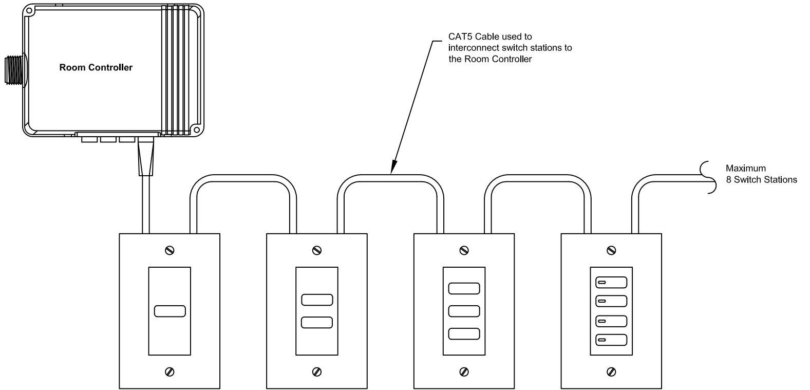
NX Switch Stations
